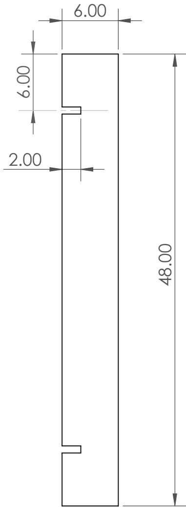
TREAD SUPPORT (3 EA)
