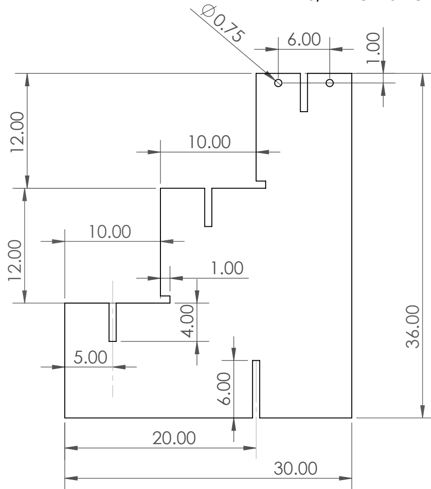
STAIR STRINGER (2 EA)
