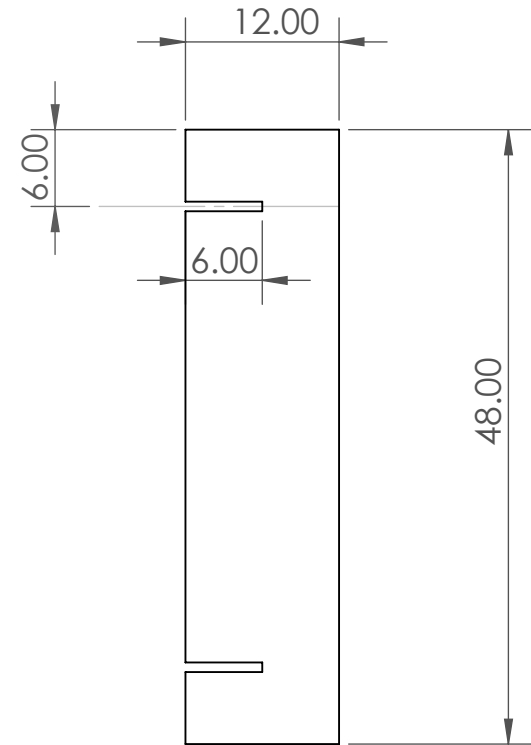
BOTTOM SUPPORT (1EA)
