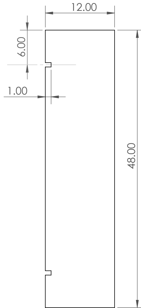
TREAD (3 EA)
